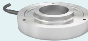
LWMH2 Large Load Washer with Mounting Holes 112.4 lbf to 4.5K lbf 0.5 kN to 20 kN
