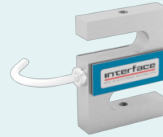
SSM-FDH Sealed High Temperature S-Type 50 lbf to 250 lbf 200 N to 1.25 kN
